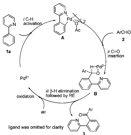
Scheme 1. Plausible Mechanism
